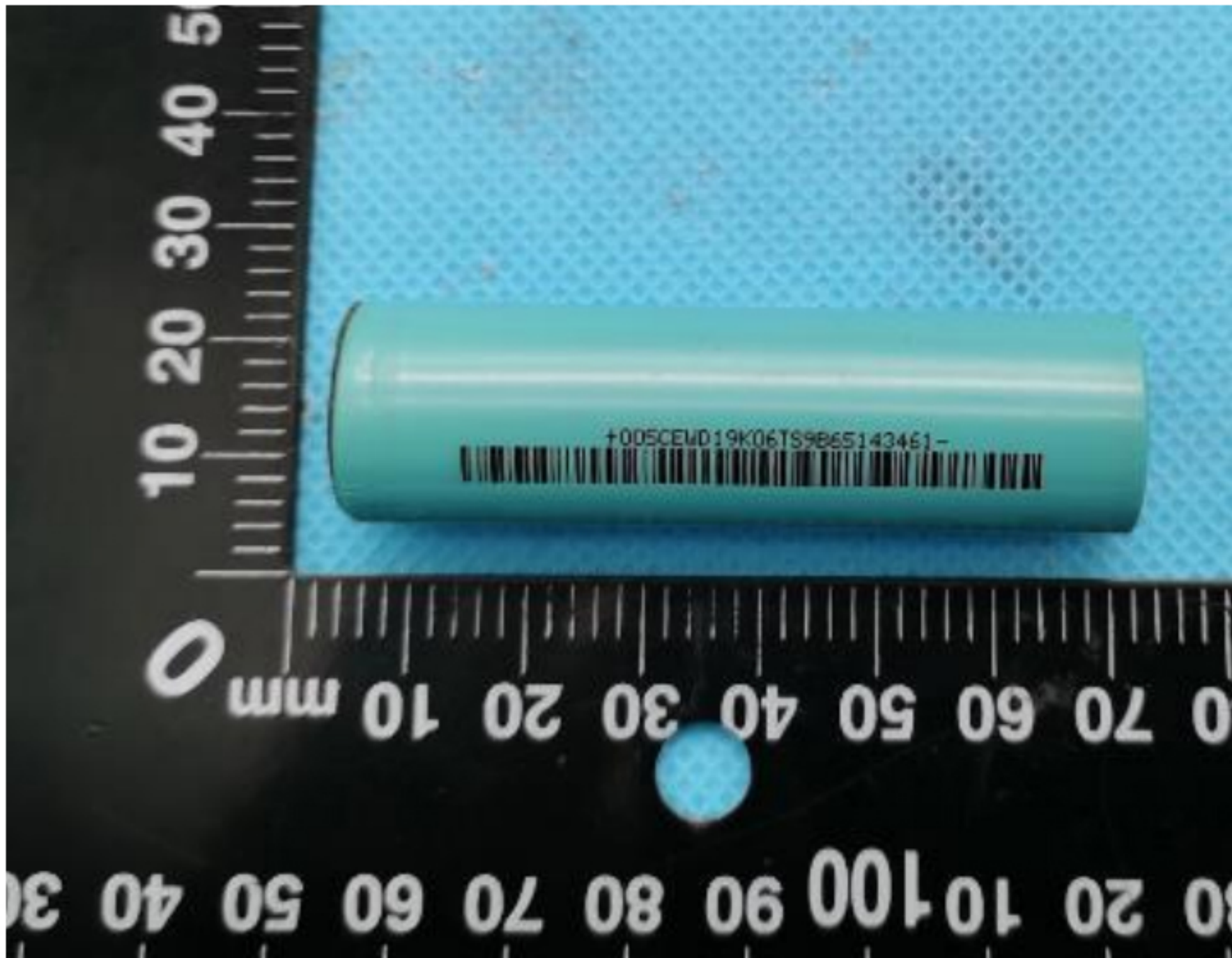
Cells /电芯 (18650 3.6V 3000mAh 10.8Wh)
