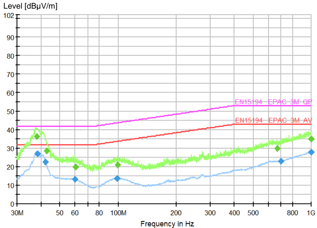
Figure 1: Spectral diagrams and measurement results, 30 – 1000 MHz, Horizontal polarization, Left side
