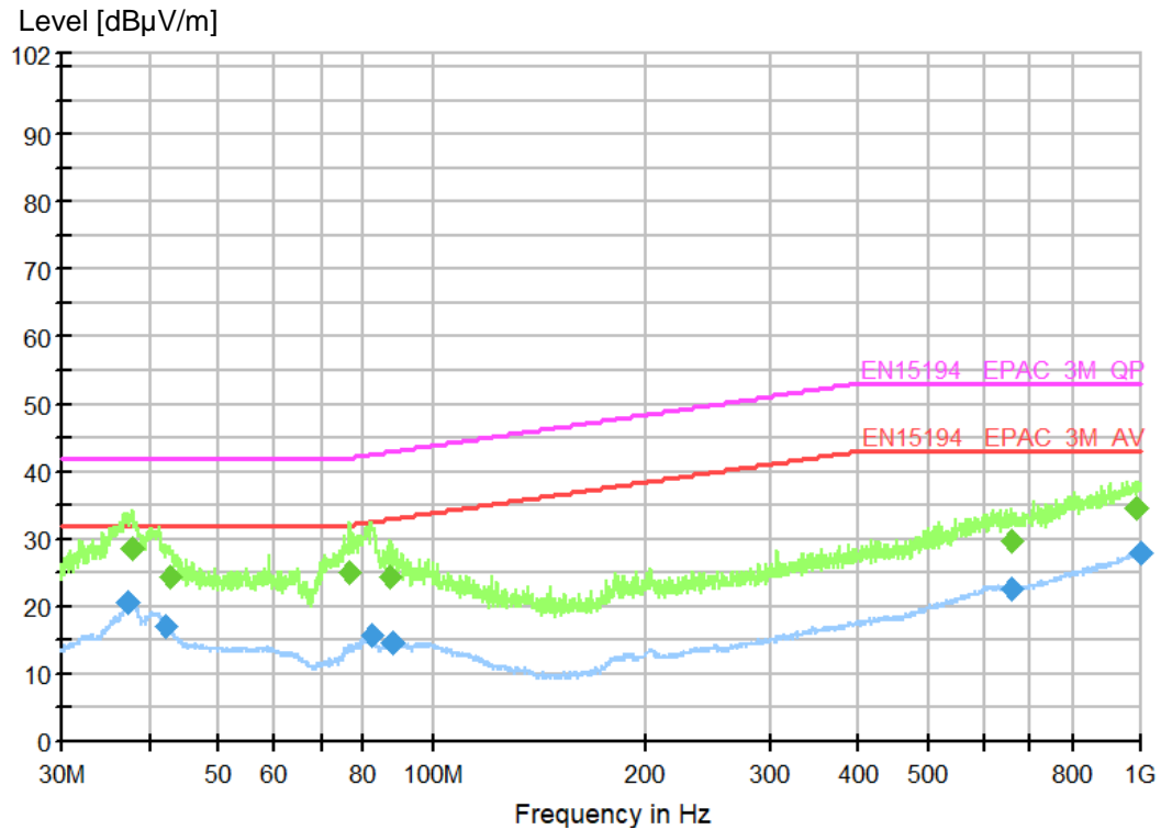
Figure 4: Spectral diagrams and measurement results, 30 – 1000 MHz, Vertical polarization, Right side
